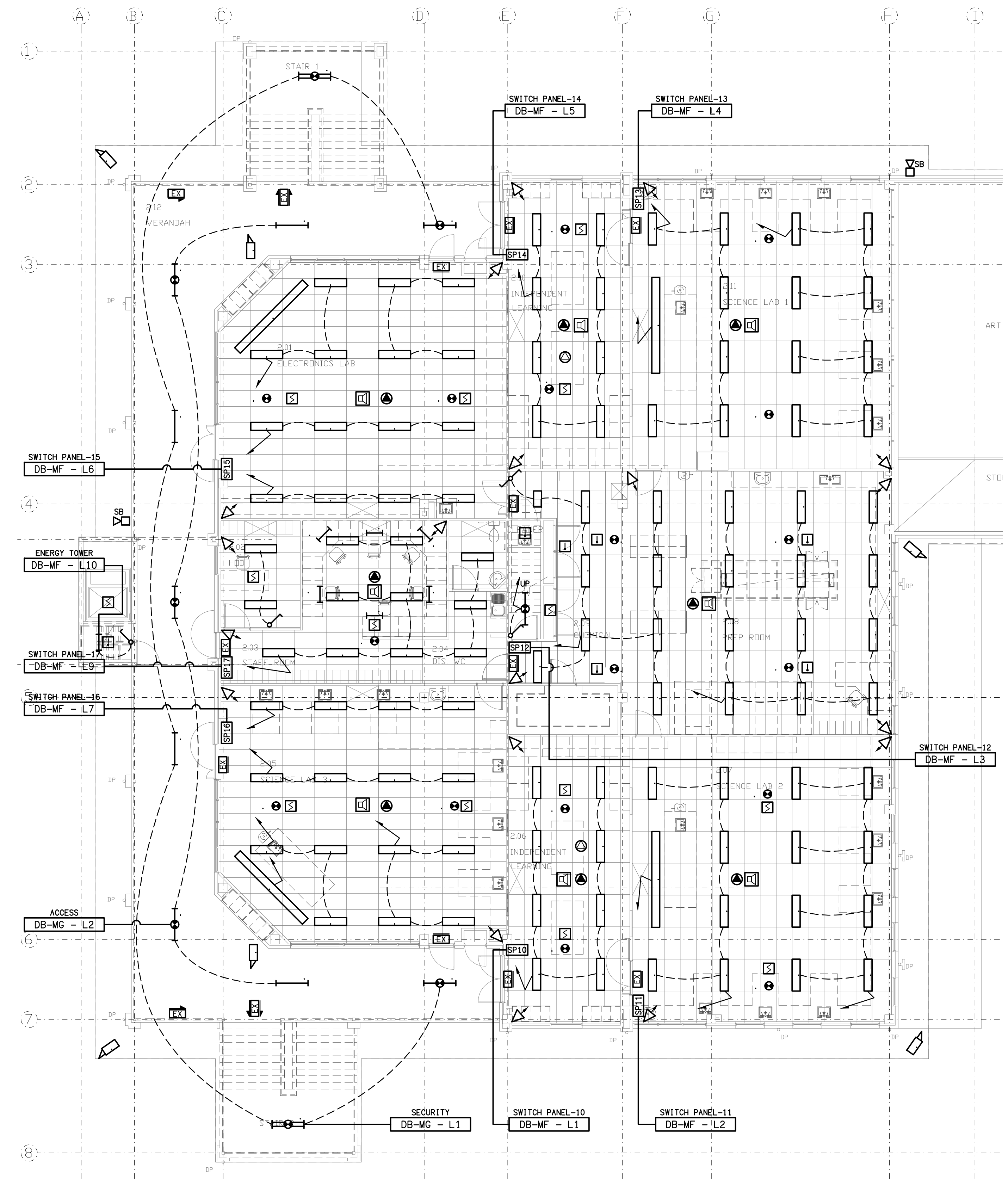
REFLECTED CEILING PLAN EXISTING LEVEL 1 SCALE 1: 100
