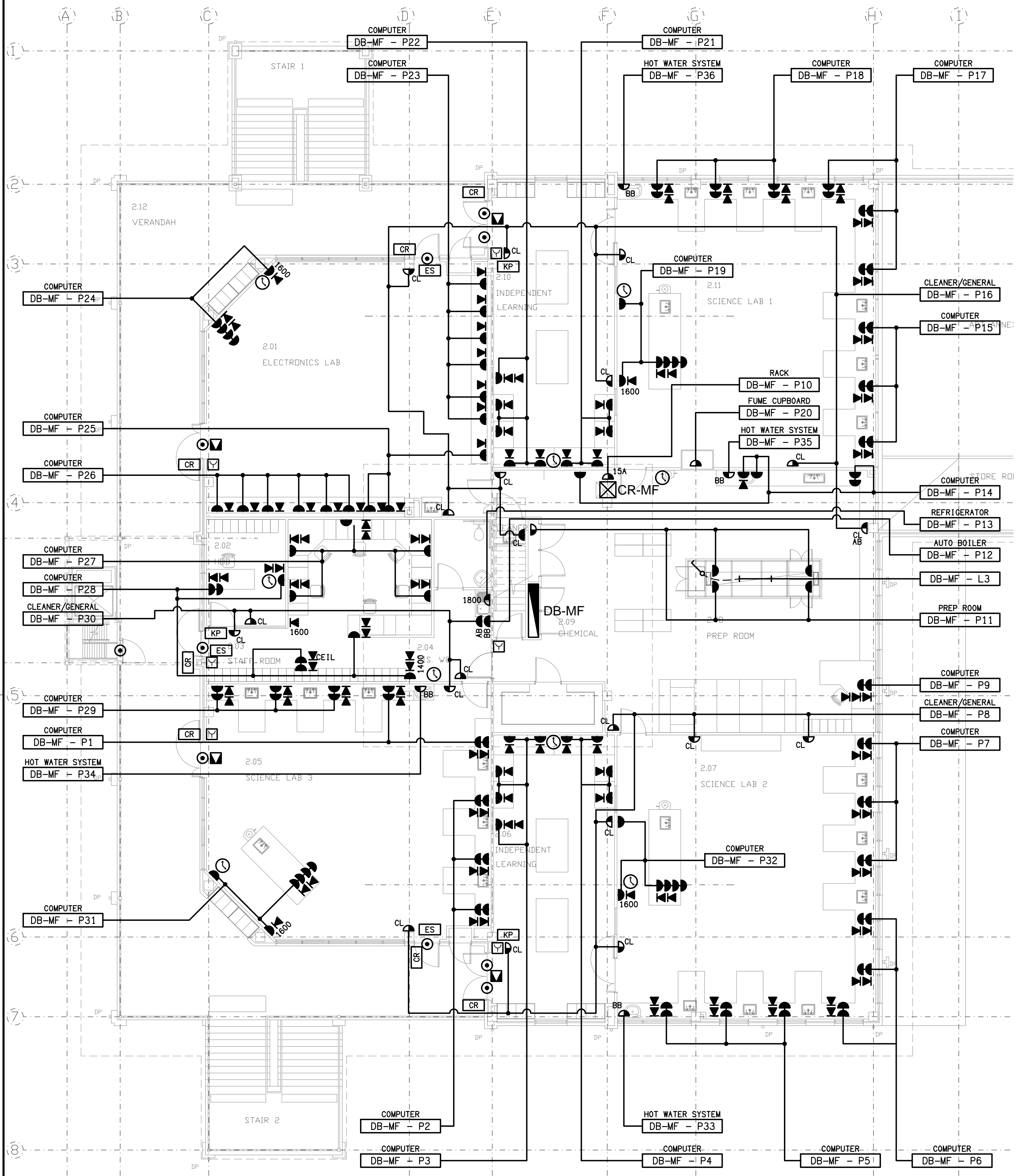
FLOOR PLAN EXISTING LEVEL 1 SCALE 1: 100
